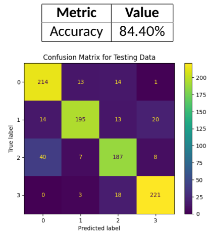
Figure 6: Confusion Matrix from the progress report.
